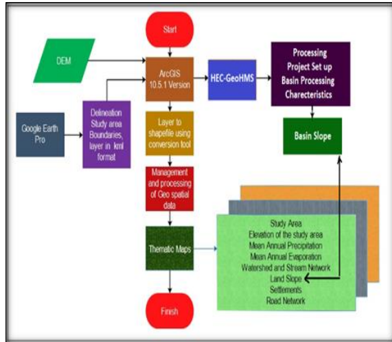
Fig. 2 Flow chart methodology remote sensing modeling.
