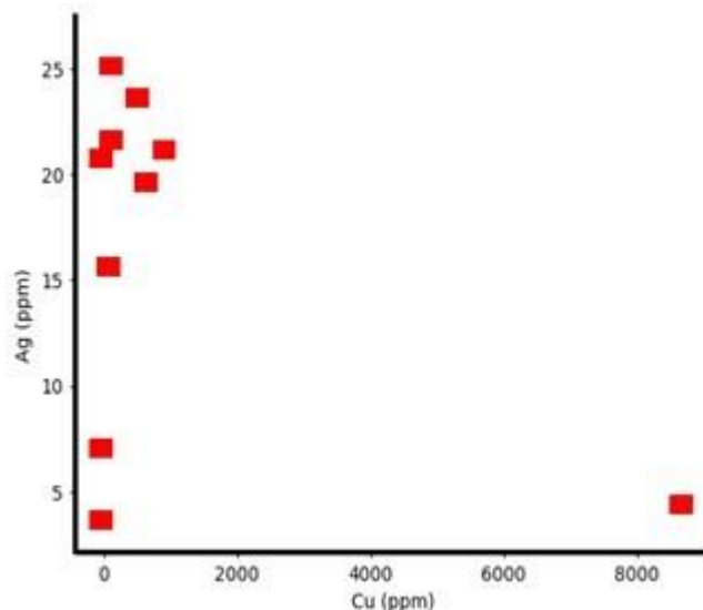
Fig. 5 Diagram for Hanzal quartz veins showing weak correlation and dispersion, reflecting magmatic-hydrothermal metal fractionation via brine-vapor separation and fluid evolution (Heinrich et al. , 1999; Sillitoe, 2010).
