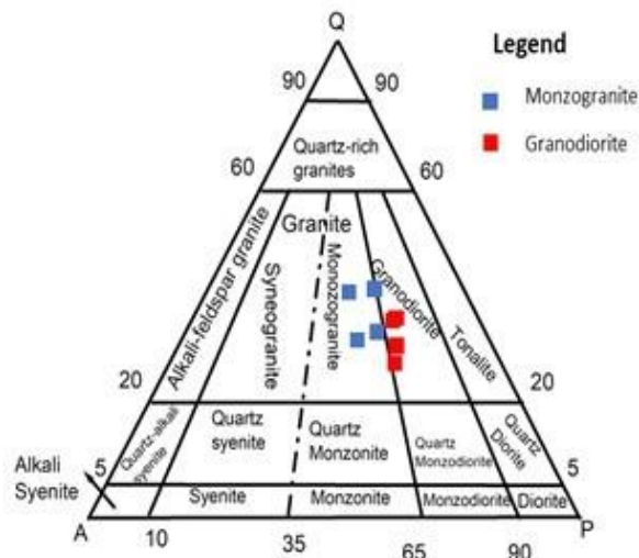
Fig. 4 Plots of modal mineralogy of granite from the Hanzal-Sorat area in Streckeisen's (1974) QAPF classification diagram for plutonic igneous rocks.
