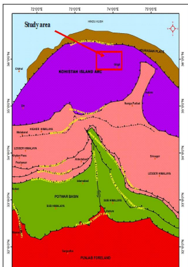
Fig. 1 Tectonic framework of Northern Pakistan (After Kazmi & Rana, 1982; Rustam & Ali, 1994; Chaudhry et al. (1997).
