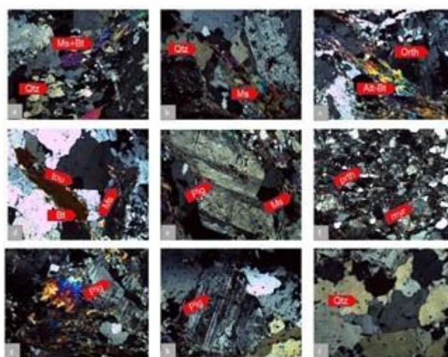
Fig. 3 Photomicrographs showing : (a) alignment of muscovite and biotite with anhedral to subhedral quartz grain in granite; (b) microcline phenocrysts surrounded by muscovite and anhedral to sub-hedral quartz crystals in Hanzal Sarot granite; (c) orthoclase in granodiorite having carlsbad twinning, and biotitic alteration; (d) tourmaline crystal with quartz grains, muscovite, biotite, and alkali feldspar in Hanzal Sarot granite; (e) biotite and quartz with zoned plagioclase, (f) myrmekite in perthite; (g) zoning in plagioclase with myrmekite in sarot granite; (h to i) plagioclase twinning and quartz grain with pyrite joint.
