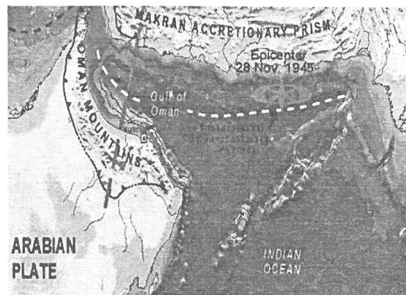
Fig 12. The Tsunami of 28 November 1945 along the Makran coast of Pakistan in the northern Arabian sea.
