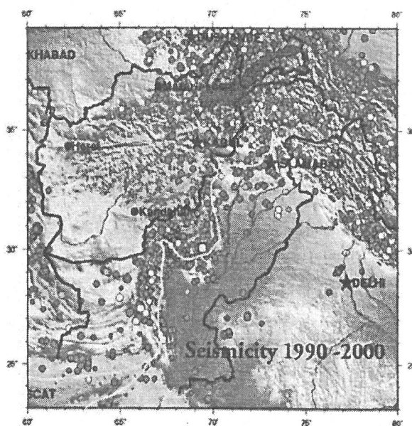
Fig 6. Northward movement of the Indian tectonic plate has resulted in major fault systems in Pakistan, Kashmir and northern India. Epicenter of the 8 October 2005 earthquake (Modified base map after Jadoon and Khurshid, 1996). Seismicity of the region from 1990-2000 (modified USGS graphic).
