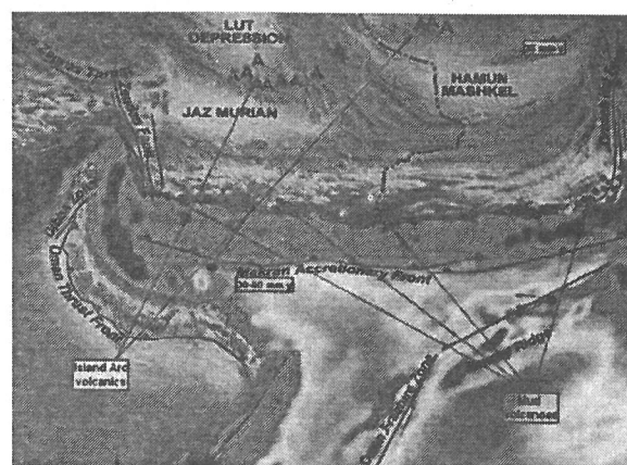
Fig 14. The Makran accretionary front. eastern and western segments - apparently discontinuous.
