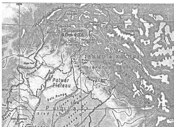
Fig 7. Physical map of northern Pakistan and of the Kashmir region affected by the 2005 earthquake.
