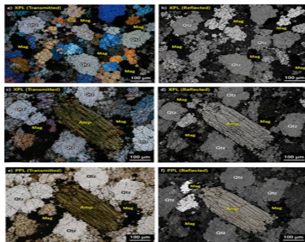
Fig. 5. Representative photomicrographs illustrating the mineralogical characteristics of selected basement core samples. Sample GDH-73/19/S-4 shows (a) transmitted light under crossed polars (XPL, 10 \times ) and (b) reflected light under crossed polars (XPL, 10 \times ). Sample GDH-74/19/S-3 displays (c) transmitted light under crossed polars (XPL, 10 \times ) and (d) reflected light under crossed polars (XPL, 10 \times ). Sample GDH-75/20/S-1 presents (e) transmitted light under plane-polarized light (PPL, 10 \times ) and (f) reflected light under plane-polarized light (PPL, 10 \times ). The photomicrographs reveal the presence of quartz (Qtz), magnetite (Mag), and amphibole (Amp).
