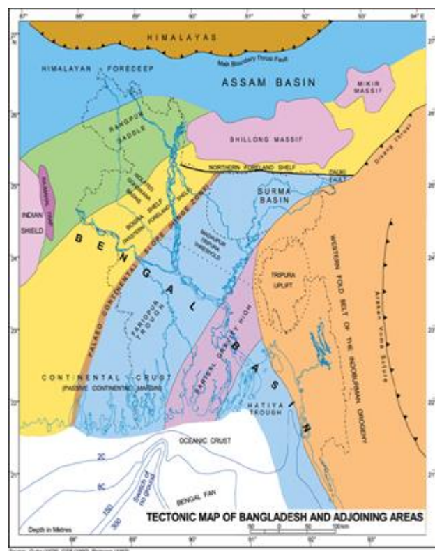
Fig. 3 Regional geological and tectonic setting of the Bengal Basin (Guha, 1978; GSB, 1990; Reimann, 1993).
