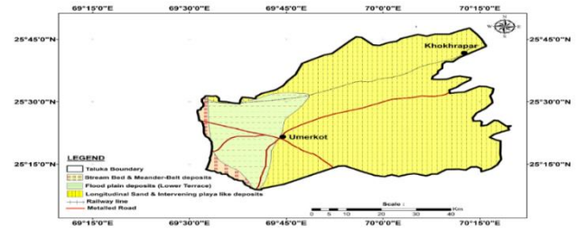
Fig. 2 Geological map of the study area (modified from Geological Map of Sindh, 2012).
