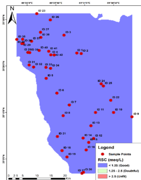
Fig. 13 Spatial distribution map of residual sodium carbonate.
