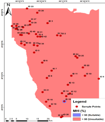
Fig. 10 Spatial distribution map of Magnesium Hazard Index.
