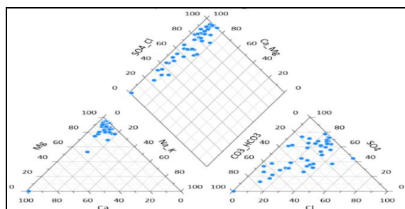
Fig. 5 Piper plot showing the hydrochemical facies of groundwater in the study area.
