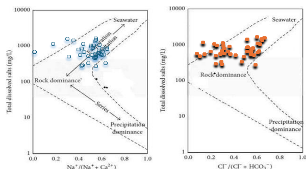
Fig. 6 Gibbs diagram showing the dominant geochemical processes controlling groundwater chemistry.
