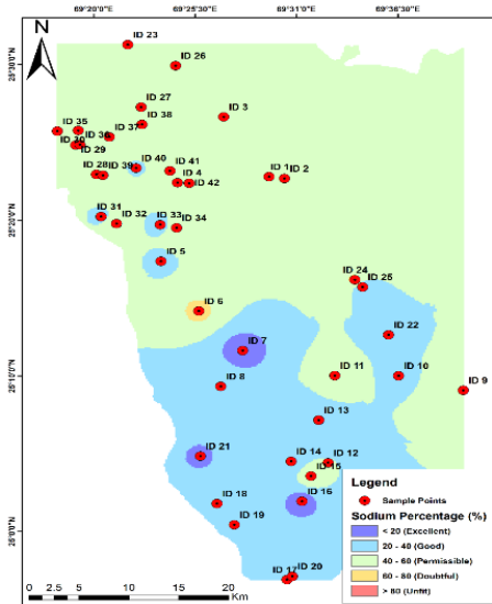
Fig. 9 Spatial distribution map of sodium percentage.
