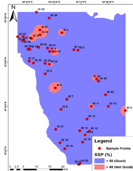
Fig. 11 Spatial distribution map of soluble sodium percentage.
