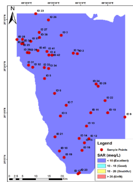
Fig. 12 Spatial distribution map of sodium adsorption ratio.
