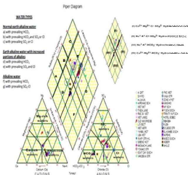
Fig. 3 Piper trilinear plot for the analysed cations and anions (Piper, 1944). Classification of hydrochemical facies using the Piper plot.
