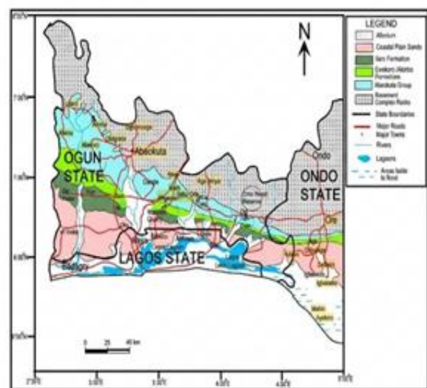
Fig. 1 Geological map of Dahomey Basin in the Nigerian sector and the states located on the basin (Olabode & Mohammed, 2016).
