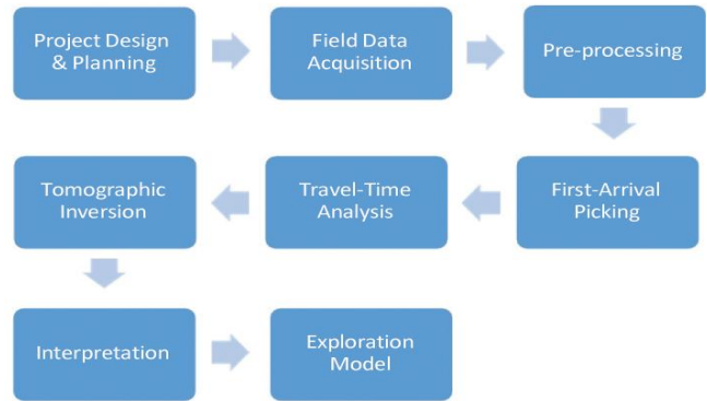
Fig. 3 Flowchart of Seismic Data Acquisition, Processing and Interpretation.
