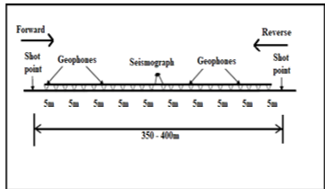
Fig. 4 Adopted data collection profile line.
