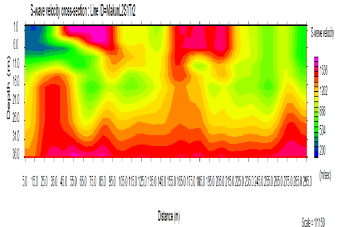
Fig. 7d S-wave cross section from Makun.
