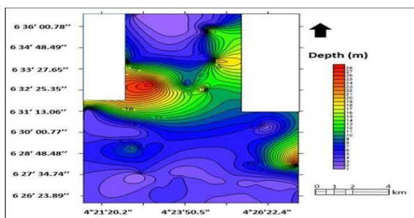
Fig. 8a Map of depth to bituminous sand layer for horizon 1.
