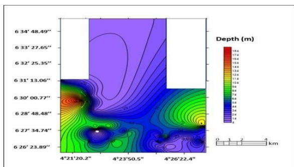
Fig. 8b Map of depth to bituminous sand layer for horizon 2.
