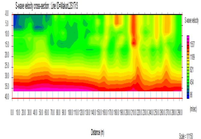
Fig. 7c S-wave cross section from Makun.
