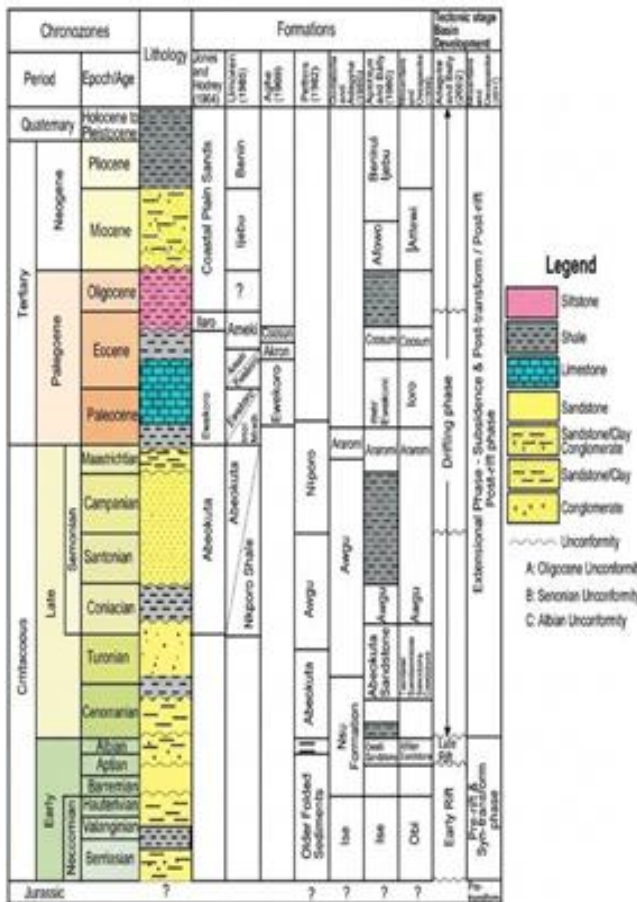
Fig. 2 Generalized stratigraphic column and tectonic stage of basin development in the Nigerian sector of the Dahomey Basin (Olalode & Mohammed, 2016).
