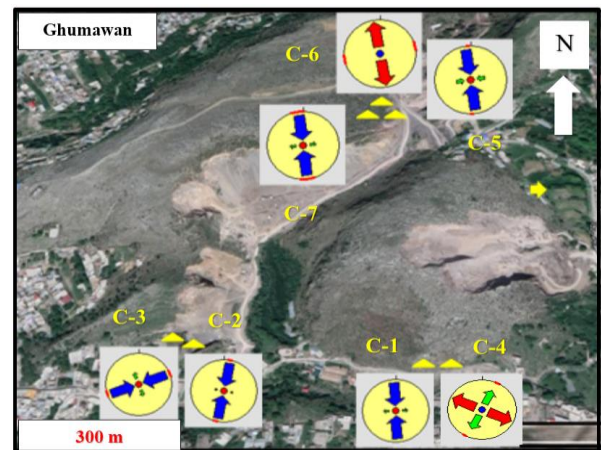
Fig. 10 Overall Win-Tensor results plotted on google imagery. It shows the orientation of the fracture pattern of the measured circles that developed in the study area.
