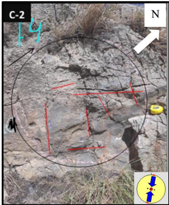
Fig. 4 Circle 2 (C-2) showing medium fracture density and joint density are 7.68 \text{ m}^{-1} . Radius of the circle is 35 cm and the area is 3846.5 \text{ cm}^2 ( 0.38 \text{ m}^2 ). Two joint sets was observed.
