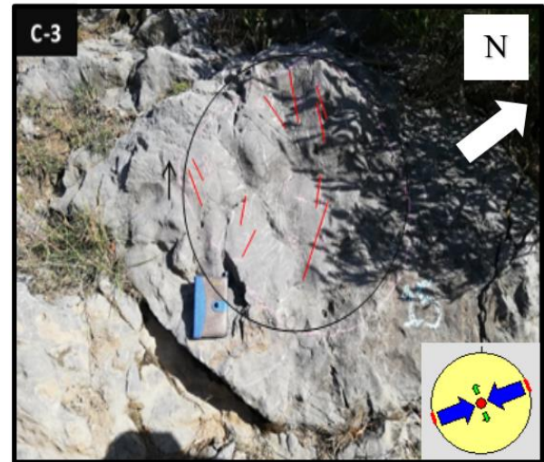
Fig. 5: Circle 3 (C-3) showing medium to high fracture density and joint density is 4.79 \text{ m}^{-1} . The radius of the circle is 35 cm and the area is 3970.5 \text{ cm}^2 ( 0.39 \text{ m}^2 ). Two joint sets were observed.
