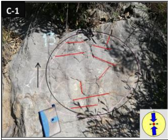
Fig. 3 Circle 1 (C-1) shows medium fracture density while joint density is 6.84 \text{ m}^{-1} . The radius of the circle is 35.5 cm and the area is 3970.5 \text{ cm}^2 ( 0.39 \text{ m}^2 ). Three joint sets were observed.
