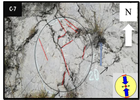
Fig. 9 Circle 7 (C-7) showing medium fracture density and joint density are 9.29 \text{ m}^{-1} . The radius of a circle is 33 cm and the area is 3420 \text{ cm}^2 ( 0.342 \text{ m}^2 ). Two joint sets are observed.
