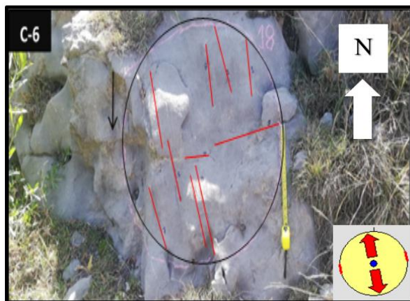
Fig. 8 Circle 6 (C-6) shows a high fracture density and joint density is 8.22 \text{ m}^{-1} . The radius of the circle is 40 cm and the area is 5042 \text{ cm}^2 ( 0.50 \text{ m}^2 ). Two joint sets are observed.
