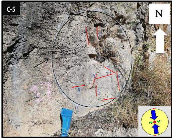
Fig. 7 Circle 5 (C-5) showing medium to high fracture density and joint density is 4.97 \text{ m}^{-1} . The radius of the circle is 35 cm and the area is 3970.5 \text{ cm}^2 ( 0.39 \text{ m}^2 ). Two joint sets are observed.
