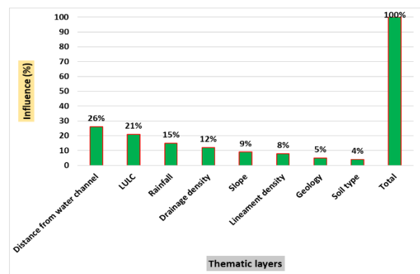
Fig. 3 weights of thematic layers used in this study for groundwater recharge.
