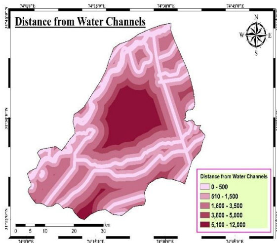
Fig. 4 Map showing distance from water channels.
