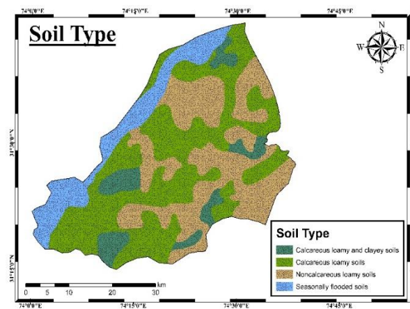
Fig. 11. Soil type map of the study area.
