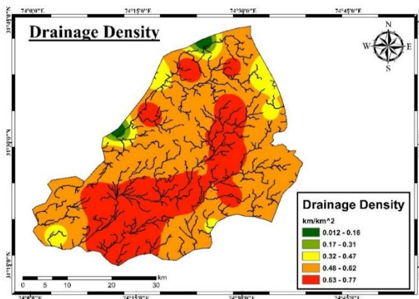
Fig. 7 Drainage density map of the study area.
