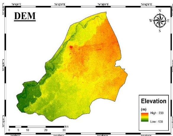
Fig. 2 SRT elevation model of study area.
