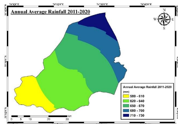
Fig. 6 Map showing annual average rainfall 2011-2020 in the study area.
