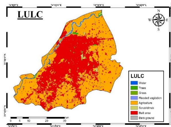
Fig. 5 LULC map of the Lahore district.
