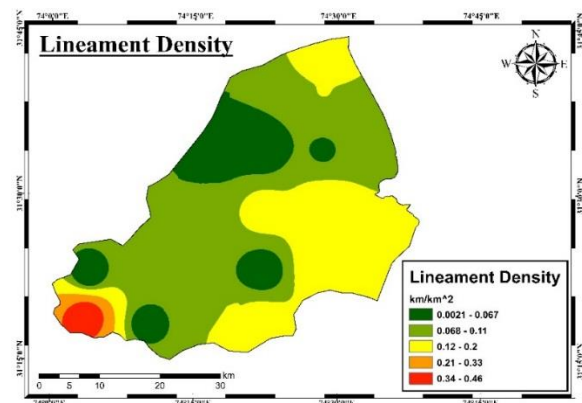
Fig. 9. Lineament density map of the Lahore district.
