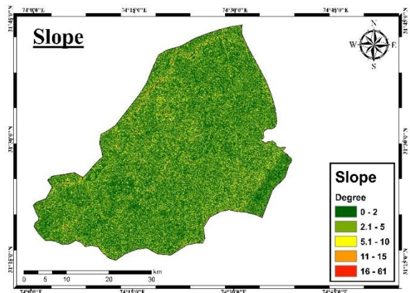
Fig. 8. Map showing the slope (degree) of the Lahore territory.
