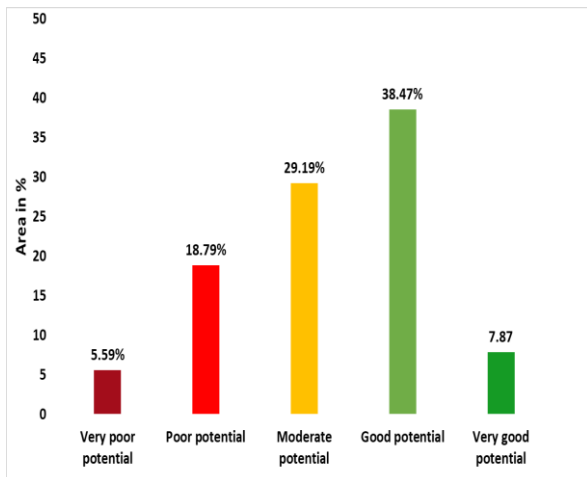
Fig. 13. % potential zones for groundwater recharge of the study area.
