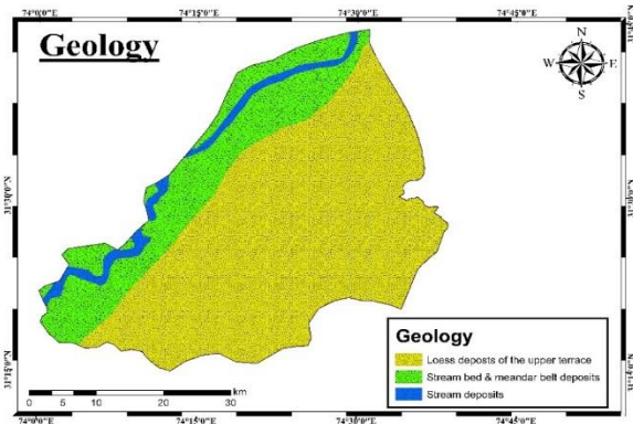
Fig. 10. Geological map of the study area.
