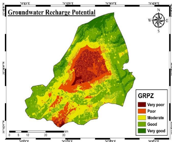
Fig. 12. Map showing the GRPZ of the Lahore district.
