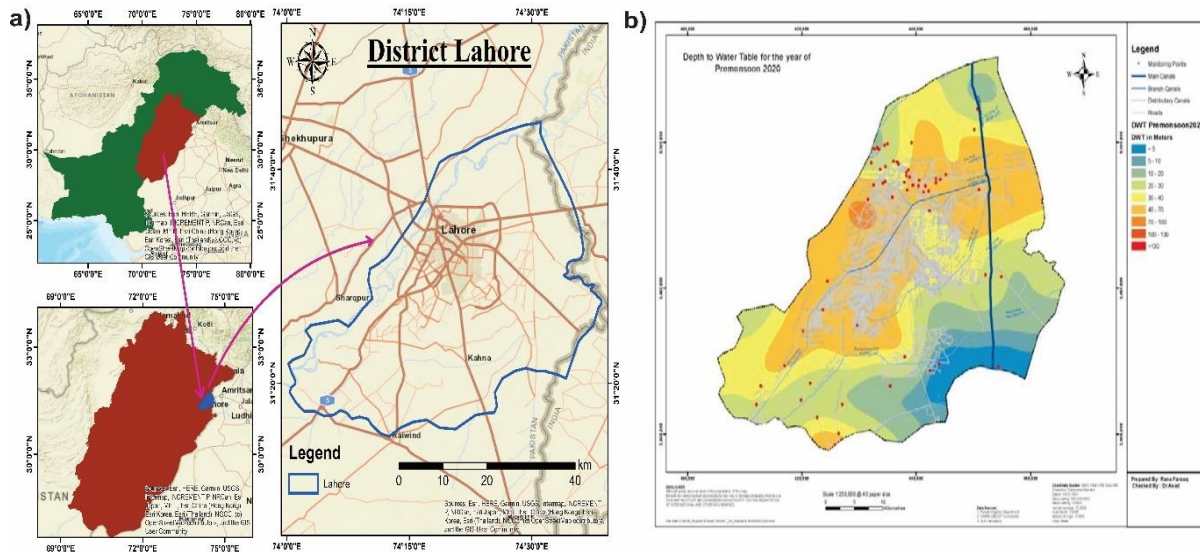
Fig 1. a) Geographic location of the study area. b) Depth to the water table for the year of pre-monsoon 2020 (Qureshi and Syed, 2014).
