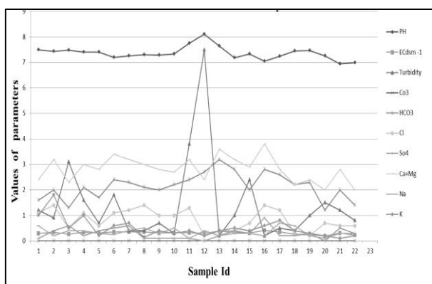
Fig. 1 Linear trend in different water parameters.
