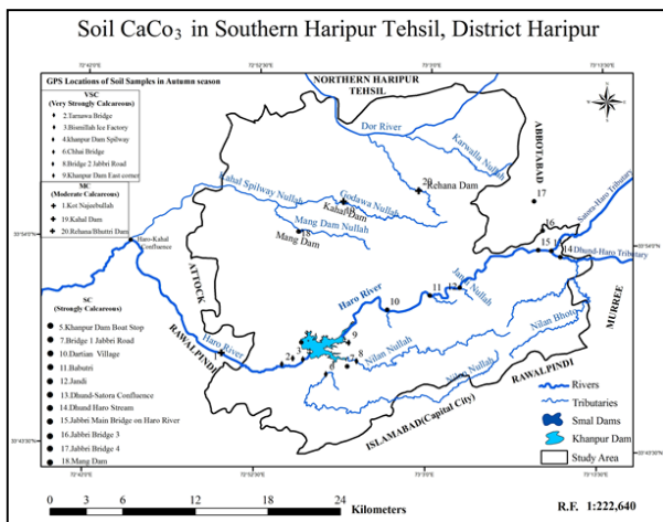
Fig. 6 Classes of \text{CaCO}_3 in study area.
