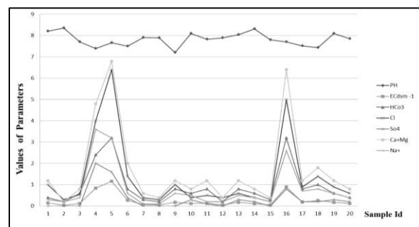
Fig. 8 Showing the linear trend in different soil parameters.
