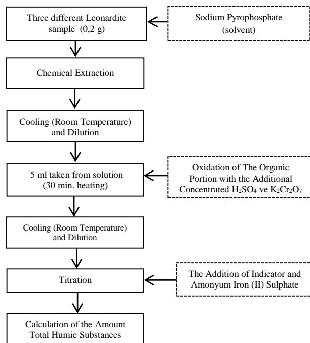
Fig. 1 The flow sheet of humic substance analysing method (TSE 5869 ISO 5073) for brown coals and lignite (Canieren, 2015).
