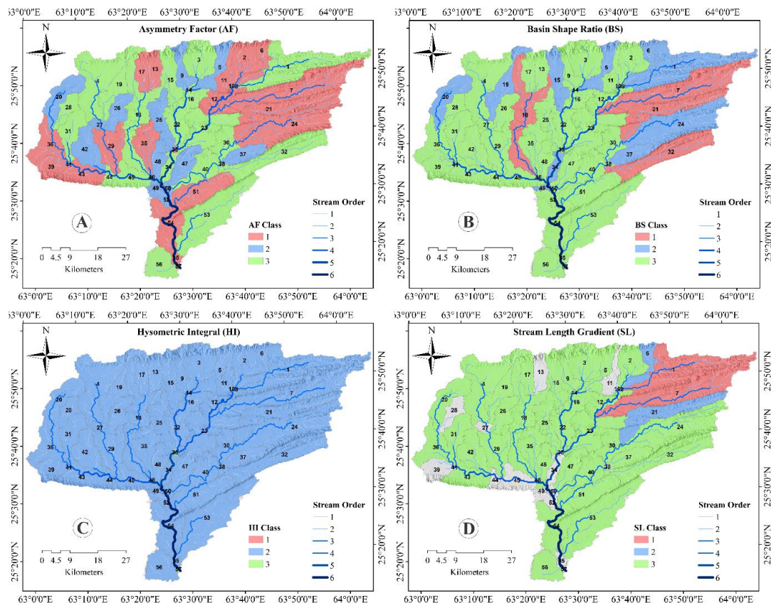
Fig. 3 Map showing the four calculated geomorphic parameters of the Shadi Kaur Catchment in Pasni at the coast of Balochistan, Pakistan (A) Factor of asymmetry, (B) shape of the basin (C) hypsometric integral, and (D) length gradient of stream. Note that the sub basins with no colors were not suitable to extract the SL index due to the threshold errors while calculating (D).
