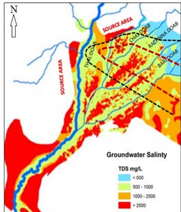
Fig. 4 Modified from map published in the IGB groundwater system report by British Geological Survey on the distribution of saline water in the IGB aquifer, (A Bell et al., 2015). The black and red dotted lines are outlines for truncations of Salt Range and Precambrian metasediments respectively around Sargodha High.
