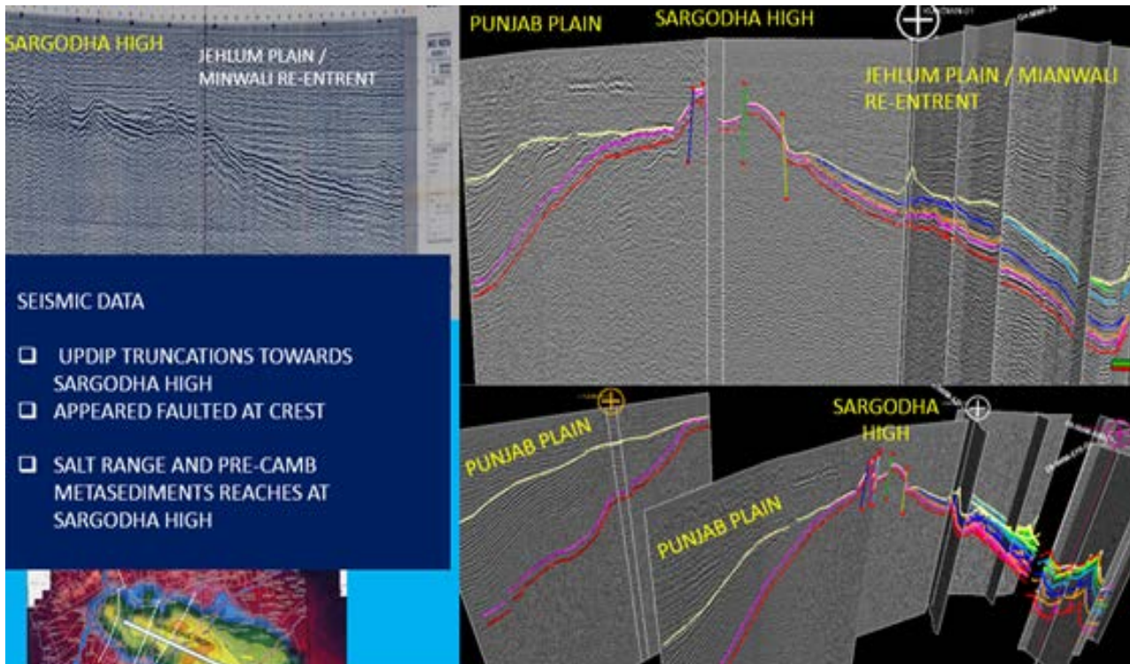
Fig. 8 Interpreted 2D-Seismic data and its correlation wells drilled for oil and gas to identify reflectors and age of rocks; white lines are showing locations of 2D data on inset map.
