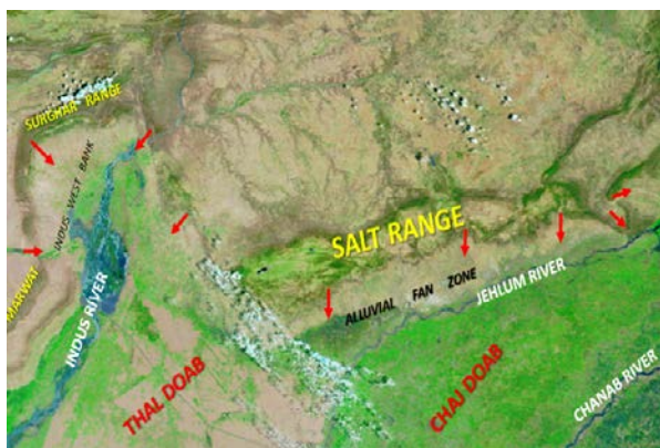
Fig. 17 Drainage zone west of Indus and north of Jhelum Rivers supplying sediments and chemically diluted fluids to soil area from Salt, Surghar and Khishore-Marwat Ranges.
