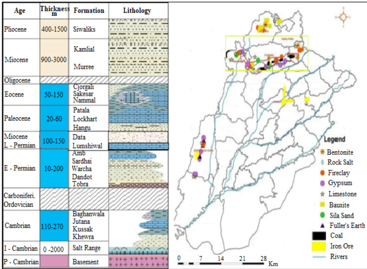
Fig. 2 Rocks and minerals reported in the surrounding hills of Doabs (modified after Malkani et al., 2017). The stratigraphic column is reporting the type of lithologies seen on Salt and Trans Indus Ranges. Yellow outline area is showing the location of Salt Range outcrops.
