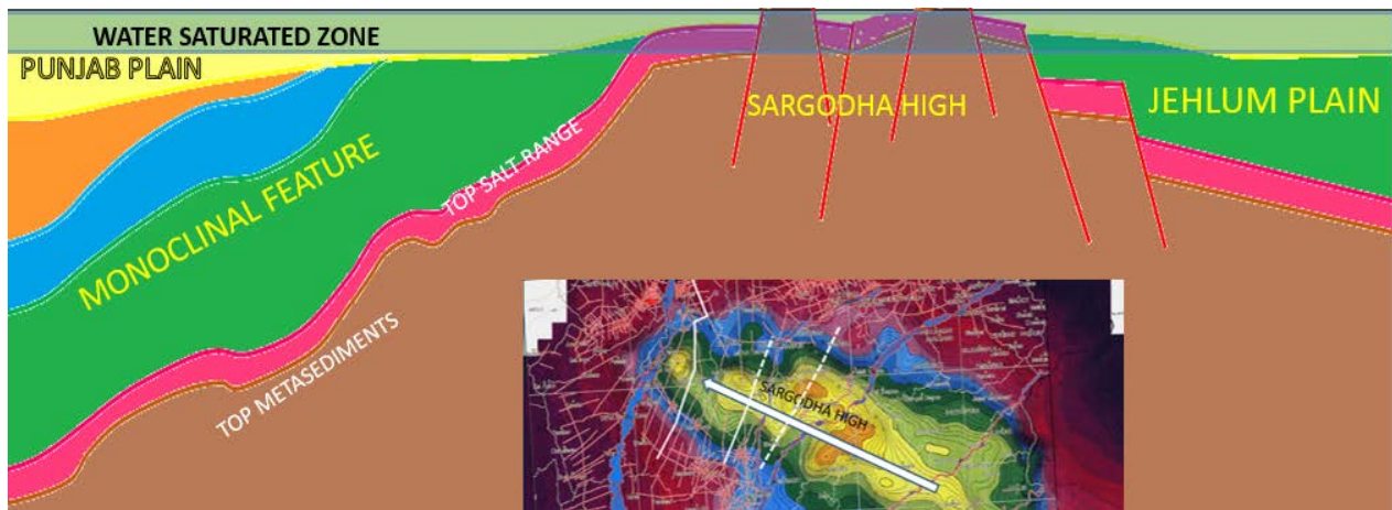
Fig. 9 Subsurface geological model of Doab areas, interpreted from 2D-Seismic, well and surface geological data, along with expected water saturated zone.
