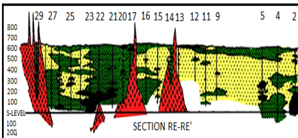
Fig. 14 EW-Geological X-section showing lithology encountered in the alluvial cover of Rachna Doab. Location is shown in Fig. 15 (Greenman et al., 1967).
