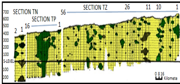
Fig. 12 Geological cross section showing lithology encountered in the alluvial cover of Thal Doab. Location is shown in Fig. 15 (Greenman et al., 1967).
