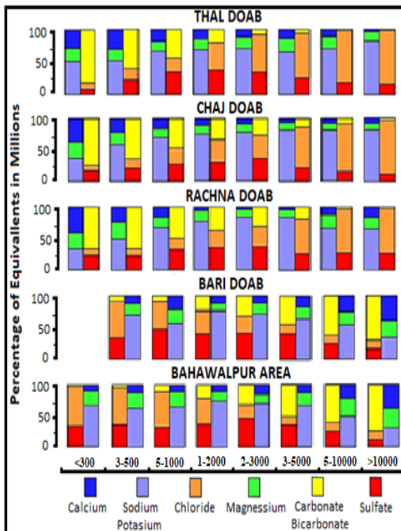
Fig. 3 Classification of GW in the Punjab region shown by bar graphs summarizing analytical data for 953 water samples taken, during WASID's test drilling operations between 1956 and 1963, from Bari, Chaj, Rechna, and Thal Doabs and the Bahawalpur area. In general, only one water sample from each test site was included in the compilation of chemical data. Figure presents a synopsis of the chemical quality of GW between depths of about 200 to 400 feet at more than 900 test sites, (Greenman et al., 1967).
