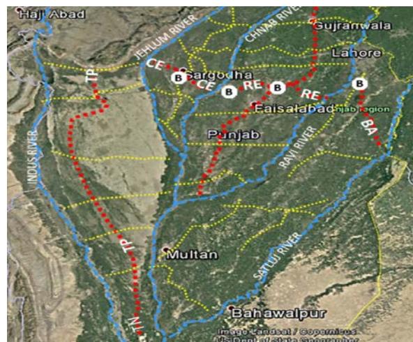
Fig. 11 Location of wells data drilled for groundwater in Doabs used to compile geological cross section. Red are major profiles along with bedrock (Precambrian Basement from Sargodha High) encountered at wells shown in white colors with symbol B. These profiles are shown in figures 14-16 (modified after Greenman et al., 1967).
