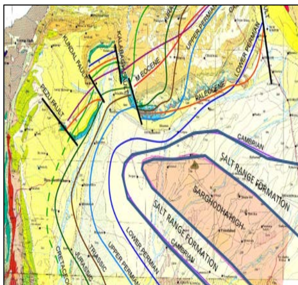
Fig. 10 Geological map with an overlay of sub-crop truncations of Precambrian, Cambrian, and Mesozoic in Punjab Plain and Potwar Basin. Presence and extent of Salt Range Formation around Sargodha High is shown and assumed from oil and gas well data (modified after Qureshi et al., 1994).
