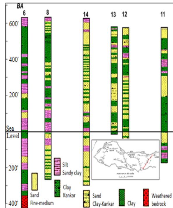
Fig. 15 Bari Doab, wells located near Lahore encountered bedrock belongs to Sargodha High (Greenman et al., 1967).
