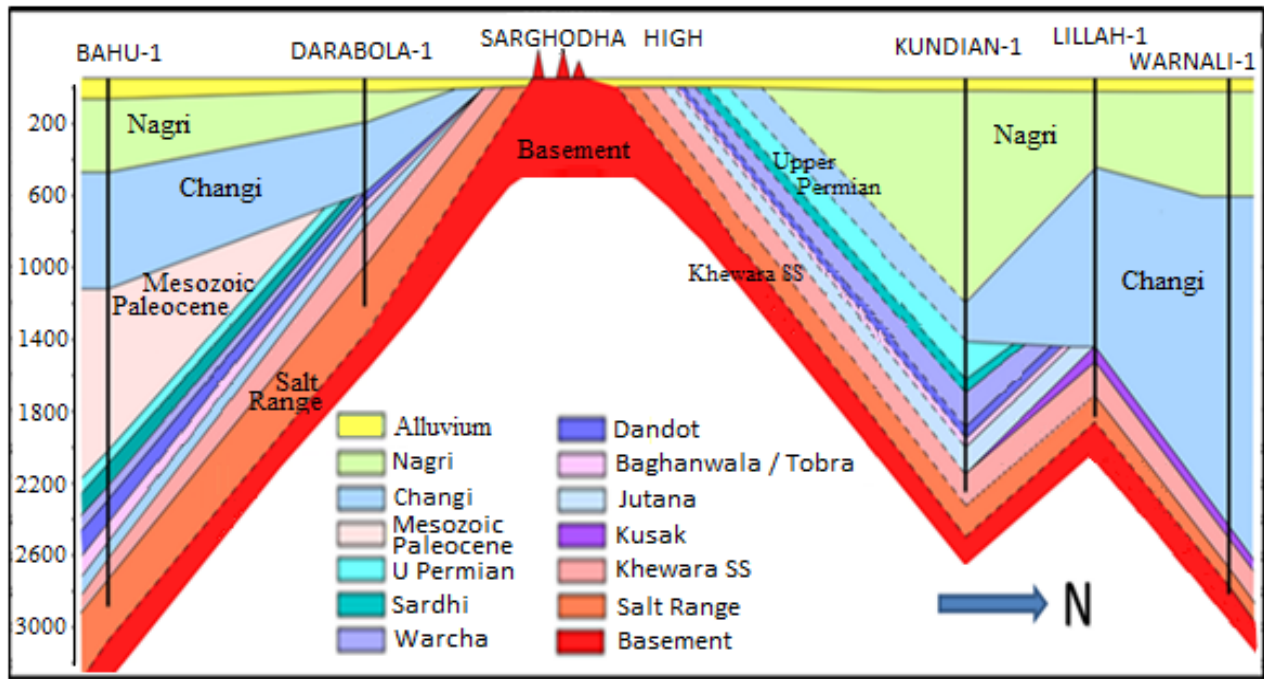
Fig. 7 X-section based on oil & gas wells data across Sargodha High showing truncation of lithological units below alluvial (yellow). Salt Range Formation intercepting alluvial in NS of Sargodha High.
