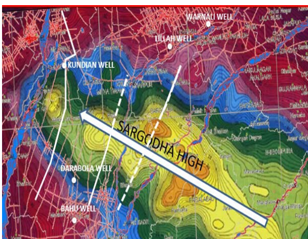
Fig. 5 Gravity map with an overlay of 2D-Seismic line location (red and white) showing Sargodha High across Doabs. White lines represent interpreted data set for model building across Sargodha High. Oil and gas wells shown by white circles, 01 (Warnali-1), 02 (Lillah-1), 03 (Kundian-1), 04 (Bahu-1), 05 (Darabola-1). The X-section of well data is shown in Fig. 8. White arrow is plunging of Sargodha High in NE direction, (modified after Philips Petroleum, 1987).
