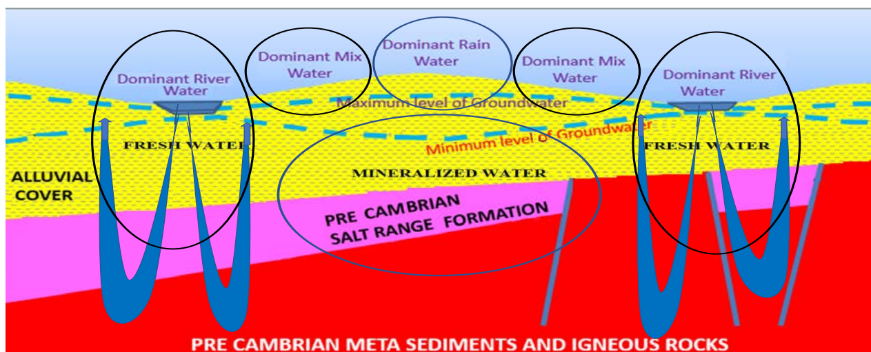
Fig. 16 Hypothetical GW model of Doabs representing near surface quality and the flow path of river water (blue arrows) from alluvial cover, underlying Salt Range, meta-sedimentary and igneous rocks.
