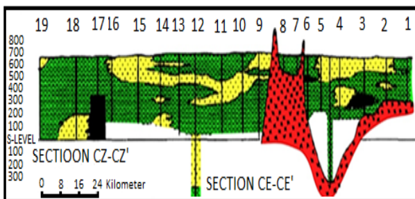
Fig. 13 Geological cross section showing lithology encountered in the alluvial cover of Chaj Doab. Locations are shown in Fig. 15 (Greenman et al., 1967).
