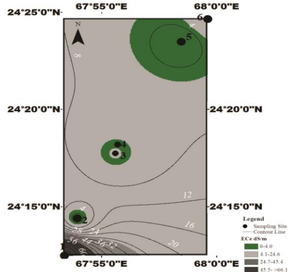
Fig. 3b. Soil Salinity (ECe) during Pre-monsoon, 2012
