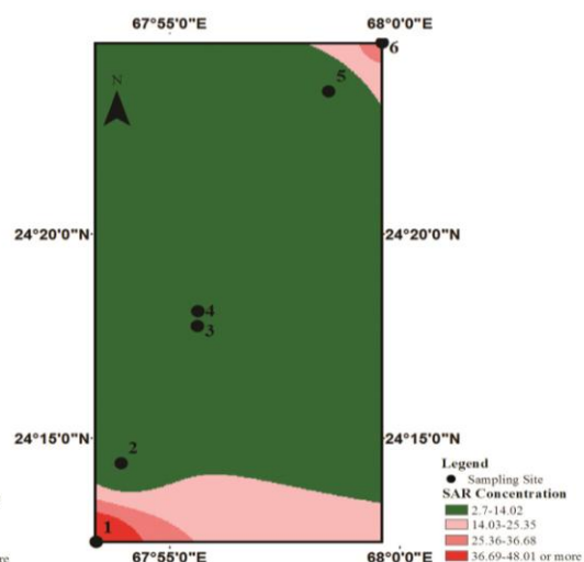
Fig. 4d. Soil Sodicity (SAR) during Post-monsoon, 2013
