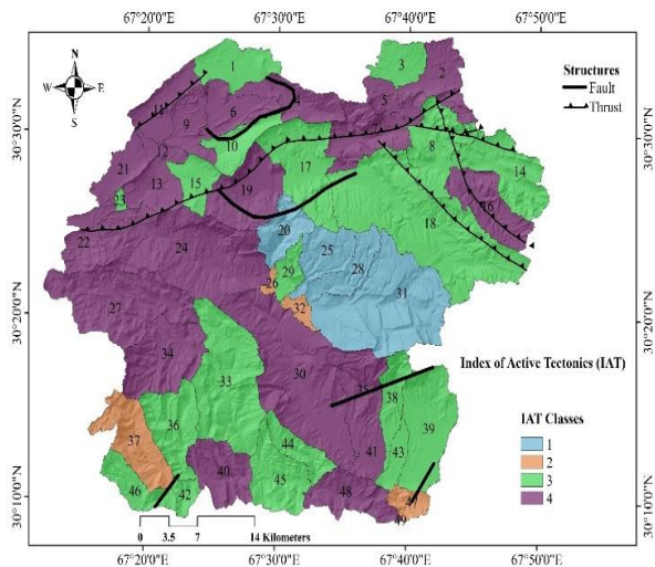
Fig. 4. Expressing the summarized four IAT classes of the Quetta-Ziarat region.
