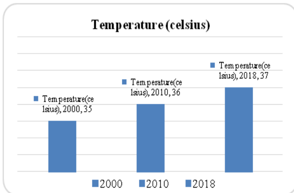
Fig 11: Average Temperature in 2000, 2010 and 2018
