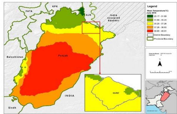
Fig 7: Temperature map of Gujarat district – 2010
