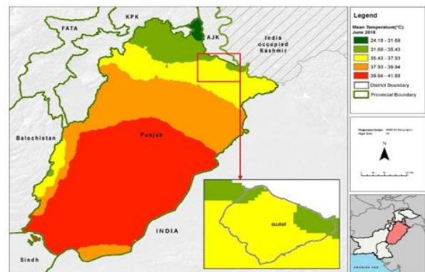
Fig 8: Temperature map of Gujarat district – 2018
