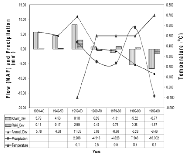
Fig. 3 Kabul river deviation from the mean flow, temperature and Precipitation.
