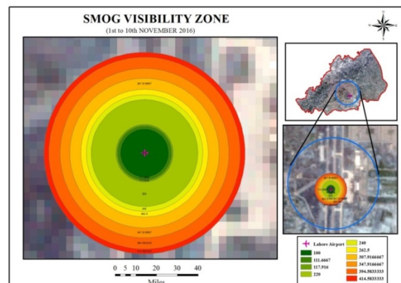
Fig. 8 Multiple buffer analysis showing smog visibility.
