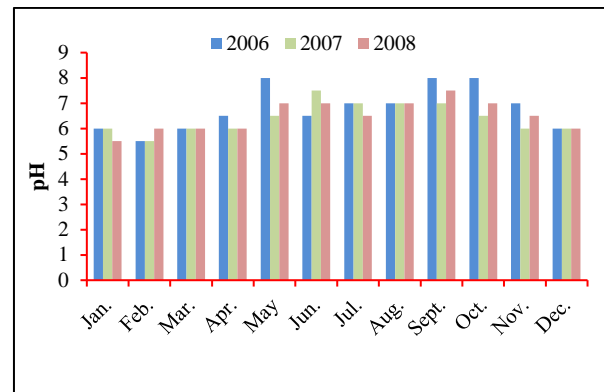
Fig. 3 Monthly variation in pH in Keenjhar lake during 2006, 2007 and 2008.
