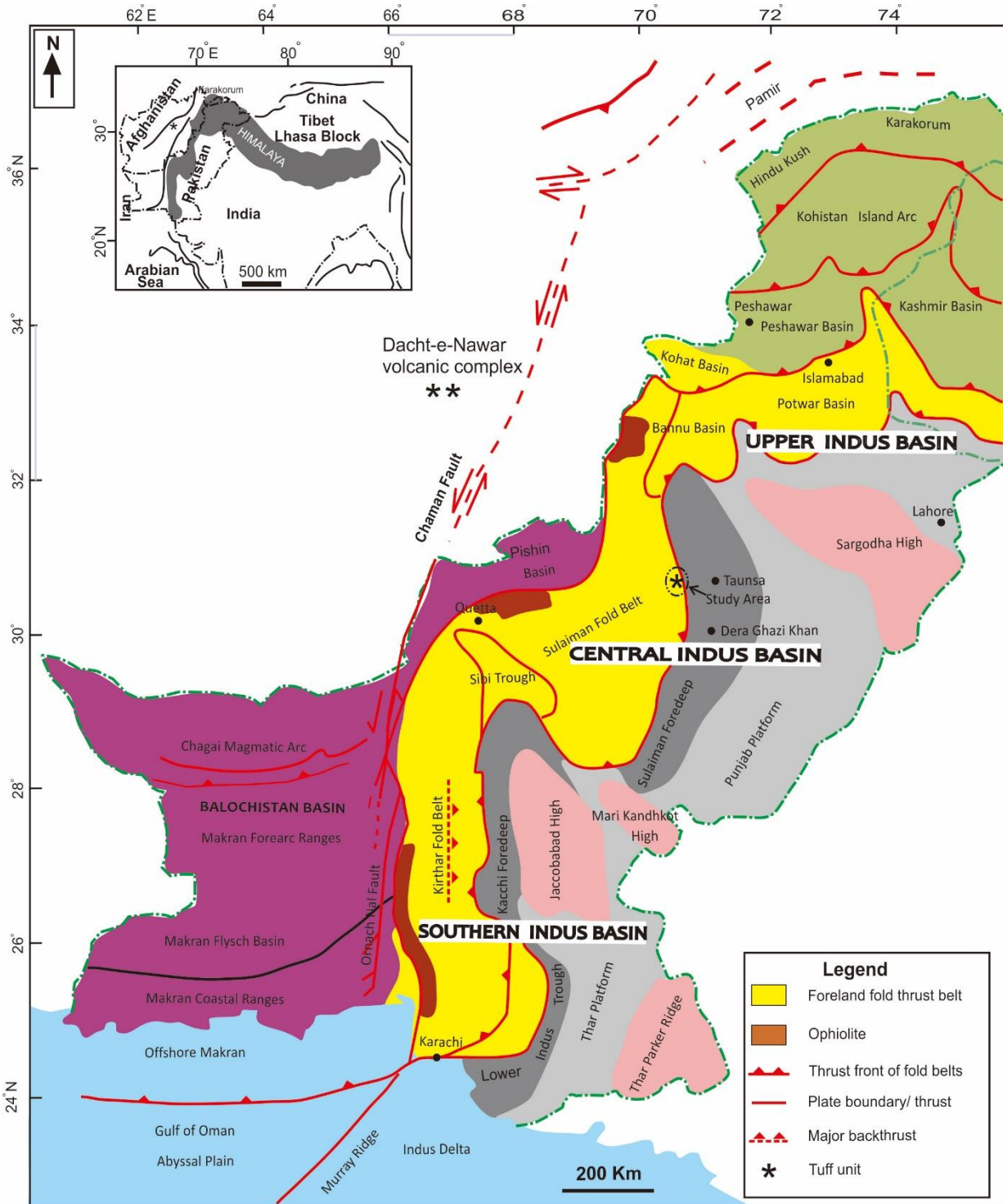
Fig. 1 Tectonic and sedimentary basin map of Pakistan (modified from Aziz and Khan, 2003). Inset shows Himalayan range and Dacht-e-Nawar volcanoes in Afghanistan (modified from Najman, 2006).
