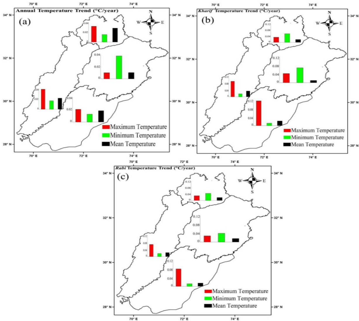
Fig. 3 Trends of temperature over the Punjab regions of Pakistan (a) Annual temperature (°C) (b) Kharif temperature (°C) (c) Rabi temperature (°C) from 1979-2019.
