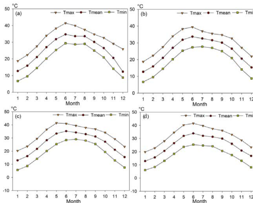
Fig. 2 Temporal patterns of temperature over the Punjab regions (a) Northern Punjab (b) Central Punjab (c) Western Punjab (d) Southern Punjab.
